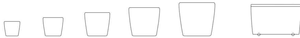
QUADRO LS 21 21×21×20 cm 8.2×8.2×7.8 in QUADRO LS 28 28×28×26 cm 11×11×10.2 in QUADRO LS 35 35×35×33 cm 13.7×13.7×13 in QUADRO LS 43 43×43×40 cm 17×17×15.7 in QUADRO LS 50 50×50×47 cm 19.6×19.6×18.5 in CARARO 75×30×43 cm 29.5×11.8×17 in
